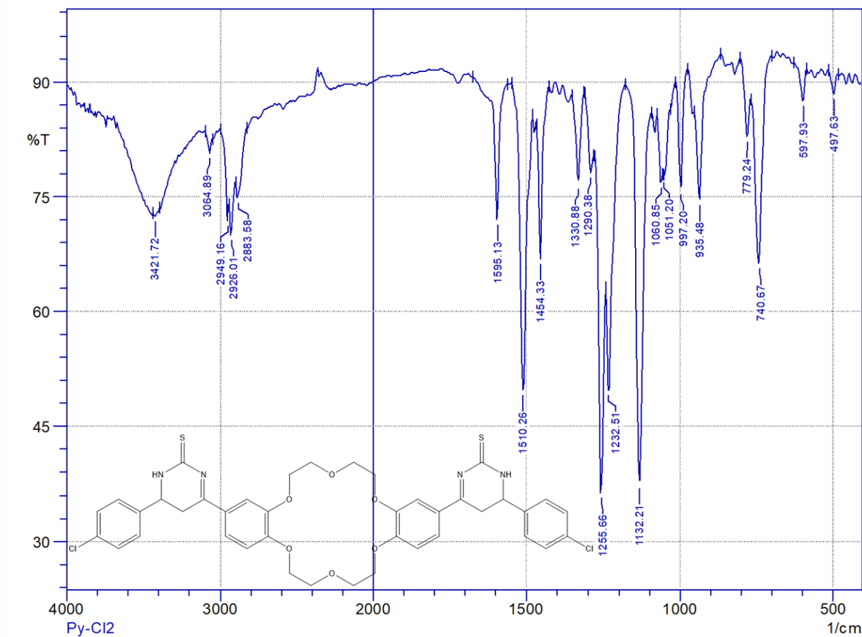
Figure 5. The FTIR Spectra of compound Z2
