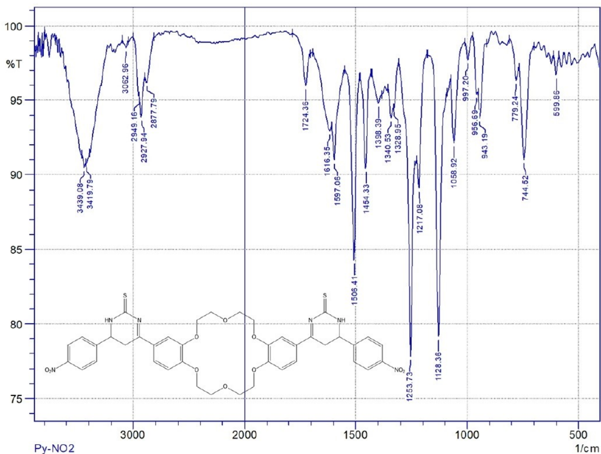
Figure 4. The FTIR Spectra of compound Z1
