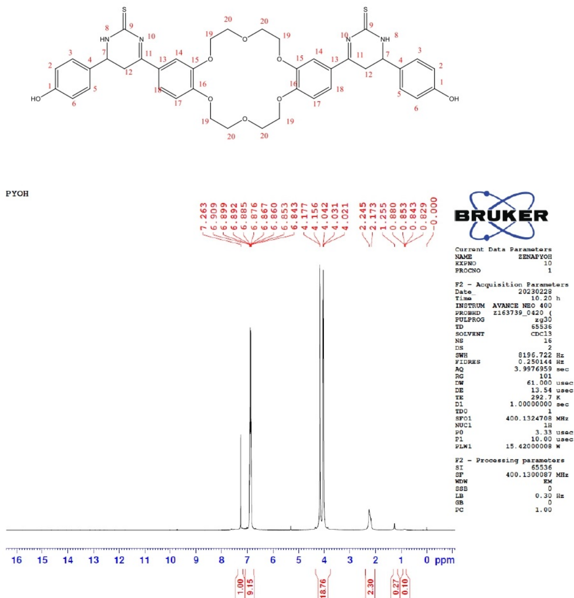
Figure 9. The ^1\text{H} NMR spectrum of compound Z3
