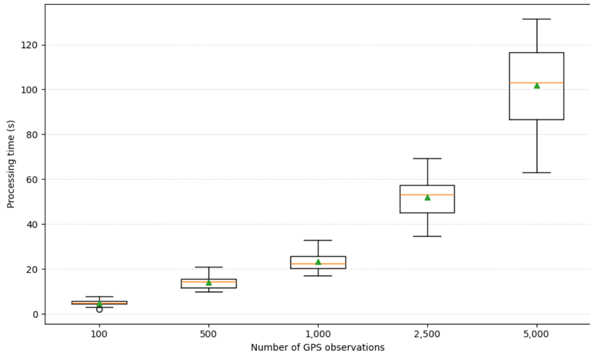
Fig. 9. Distribution of processing time across different GPS trajectory sizes
