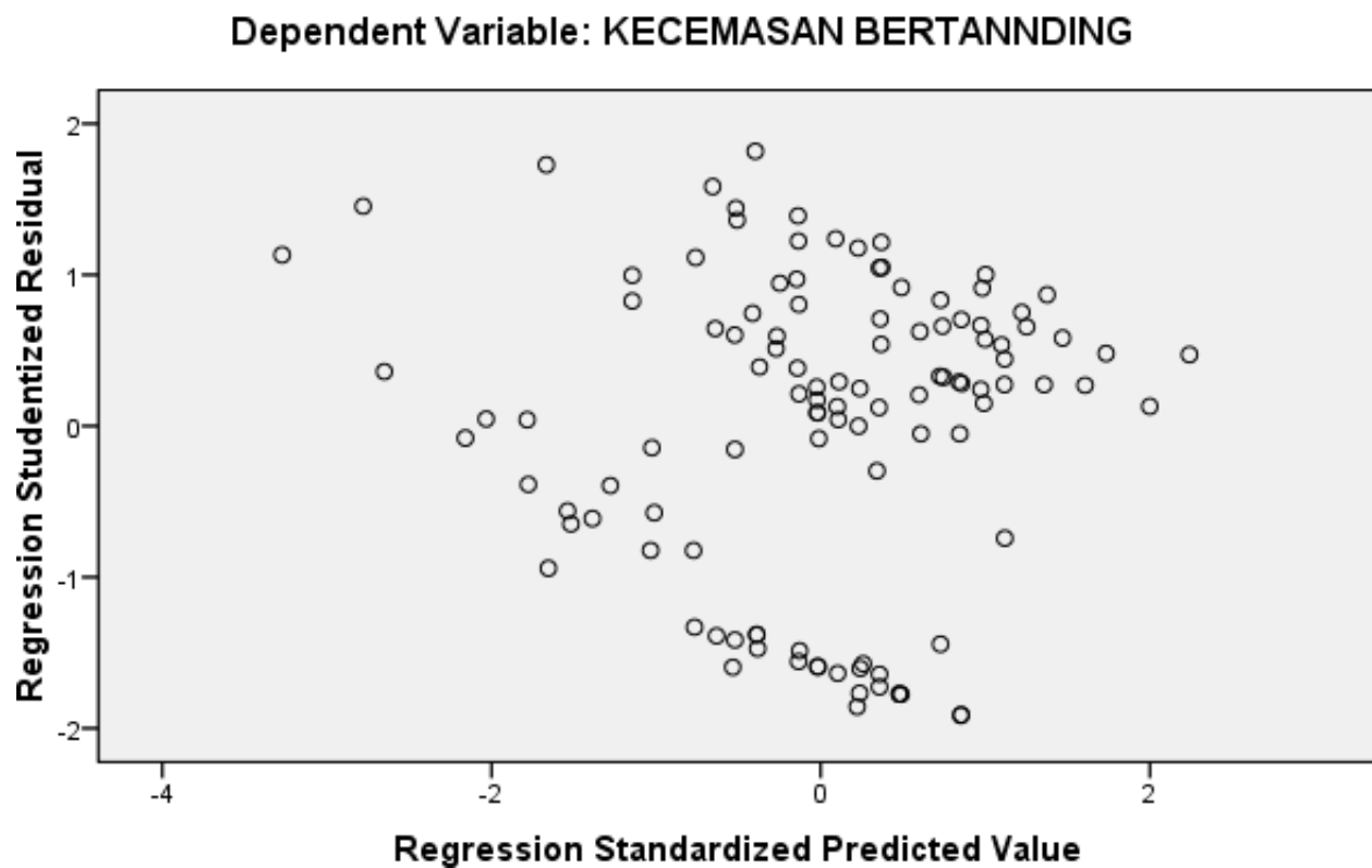
Gambar 3. Scatterplot Uji Heteroskedastisitas
