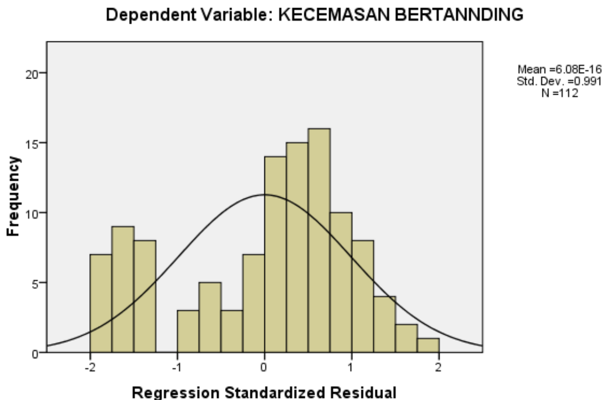
Gambar 1. Analisis Uji Normalitas Standardized Residual Histogram
